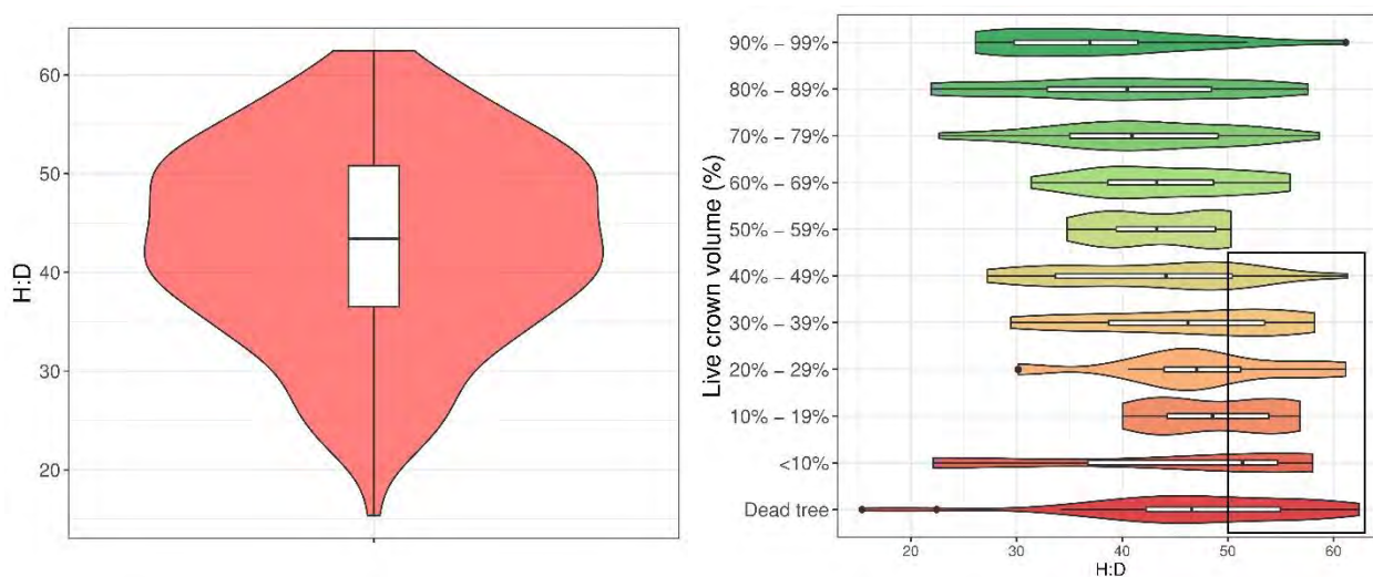
Figure 6: (left) Violin plot of Western Springs pine forest tree height to diameter ratio (H:D)
