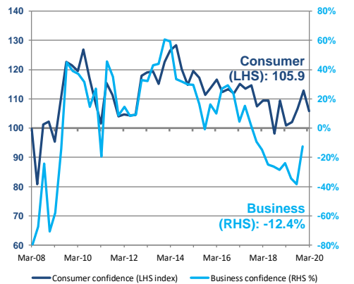
Confidence indicators 4, 5
